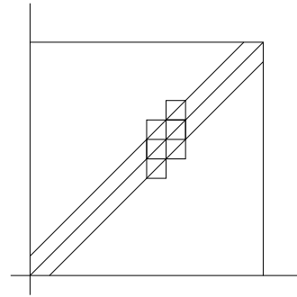
Figure 16.1. Covering by b -adic squares.
