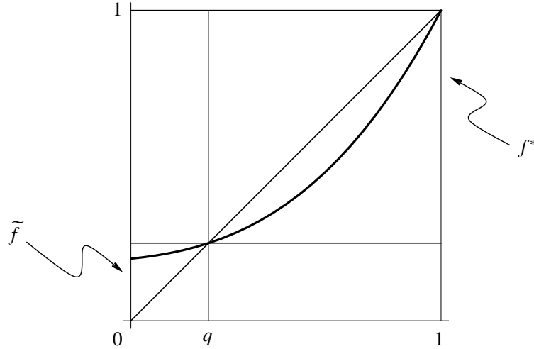
Figure 5.3. The graph of f embeds scaled versions of the graphs of \tilde{f} and f^* .
